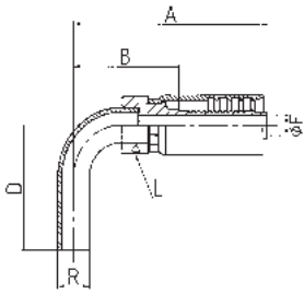
CODE N-100 METRIC STAND PIPE 90° ELBOW
