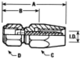
JIC 37° SWIVEL AISI 303 SERIES STAINLESS STEEL
