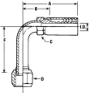
FEMALE SWIVEL, 90° ELBOW O-RING FACE SEAL (LONG DROP)
