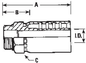
MALE O-RING STRAIGHT THREAD
