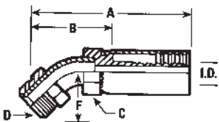
45° BENT TUBE WITH 45° INVERTED FLARE SWIVEL
