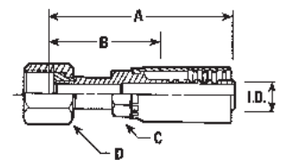
STRAIGHT WITH FEMALE SWIVEL, O-RING FACE SEAL
