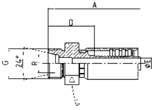
CODE S METRIC MALE RIGID (DIN 3901-3902)
