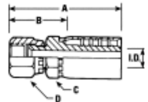
JIC 37° FEMALE SWIVEL BRASS
