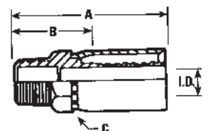
MALE PIPE RIGID BRASS
