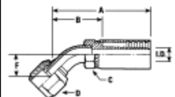
FEMALE SWIVEL, 45° ELBOW O-RING FACE SEAL
