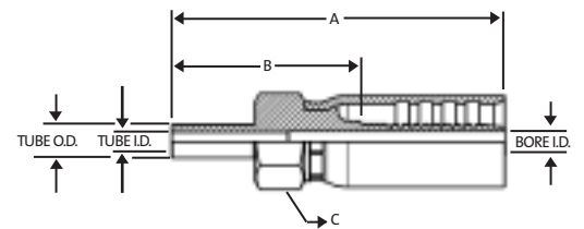
STAND PIPE, STRAIGHT, STAINLESS STEEL
