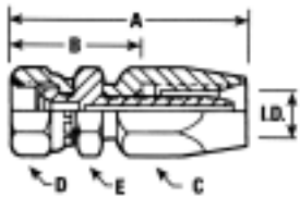
JIC 37° FEMALE SWIVEL
