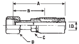
STRAIGHT WITH FEMALE SWIVEL, O-RING FACE SEAL
