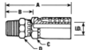
MALE PIPE SWIVEL
