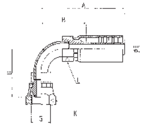
Code B-100 FEMALE SWIVEL WITH O-RING, 90° ELBOW - BSP THREAD
