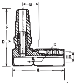
MALE PIPE SWIVEL 90° ELBOW
