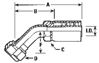
45° BENT TUBE FEMALE SWIVEL, JIC 37°
