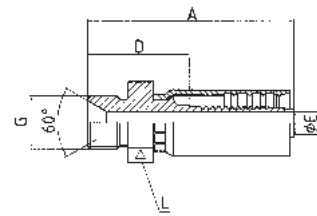
CODE Q BSP MALE RIGID
