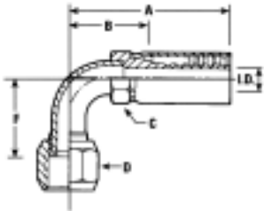
FEMALE SWIVEL, 90° ELBOW O-RING FACE SEAL (SHORT DROP)
