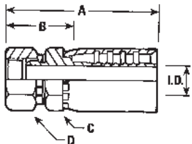
30° INVERTED FLARE NPSM
