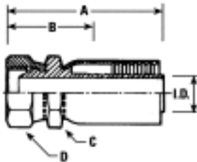
JIS FEMALE SWIVEL 60° MALE CONE (PF)
