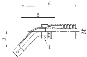
CODE N-300 METRIC STAND PIPE, 45° ELBOW
