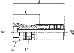
CODE B FEMALE SWIVEL, WITH O-RING, BSP THREAD
