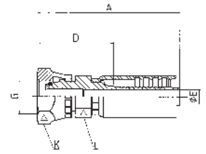
Code J-XXO FEMALE SWIVEL O-RING, METRIC THREAD
