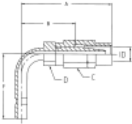
METRIC STAND PIPE 90° ELBOW (Grease Hose Series)
