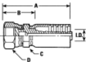
JIS FEMALE SWIVEL 60° FEMALE CONE (PF)
