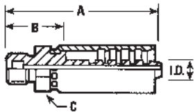
SAE FLARELESS MALE END
