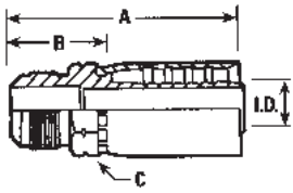
SAE 45° MALE RIGID
