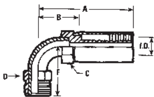
90° BENT TUBE WITH SAE 45° INVERTED FLARE SWIVEL
