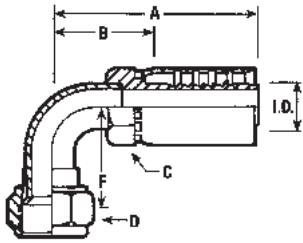
90° SHORT BENT TUBE FEMALE SWIVEL, JIC 37°
