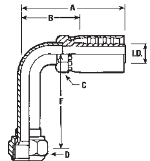
90° LONG BENT TUBE FEMALE SWIVEL, JIC 37°
