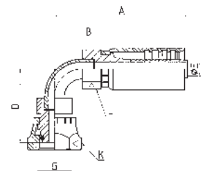
CODE J-XX1 FEMALE SWIVEL O-RING - ELBOW 90° - METRIC THREAD
